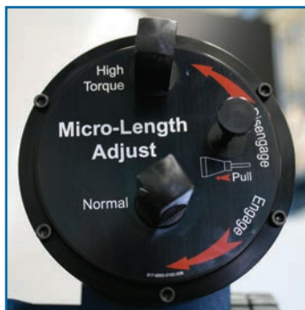
Micro Length Adjust Assembly 2 Speeds for Fine Force Adjustments
